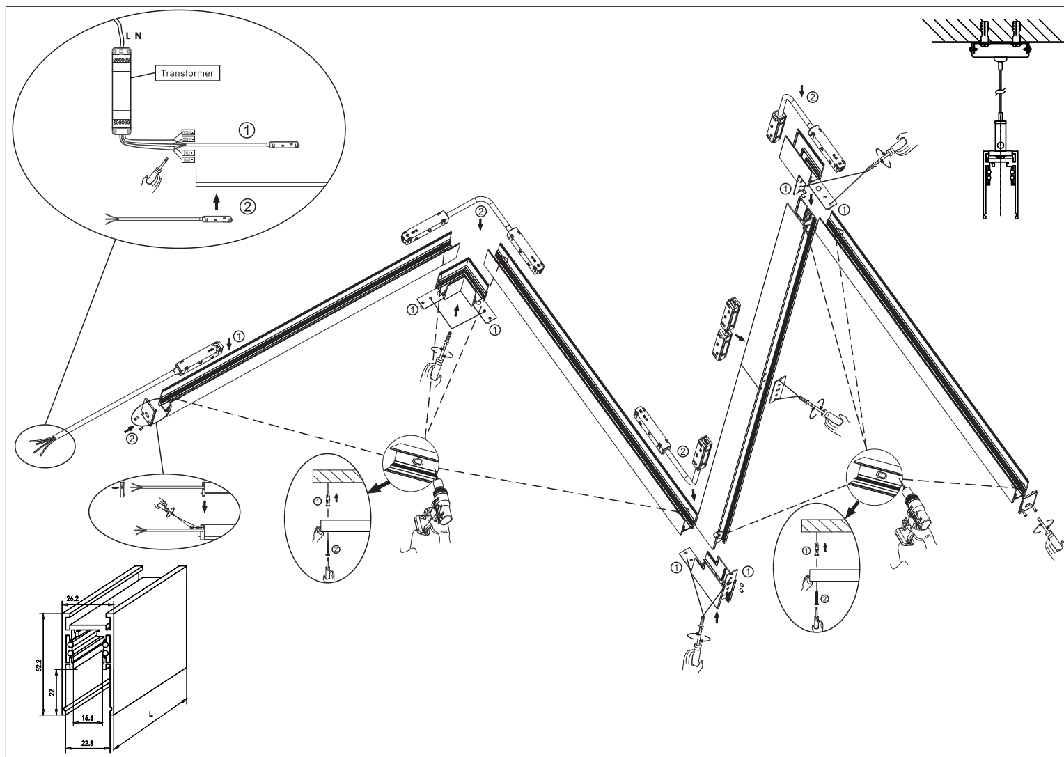
ZL-48VTR-FEEDER-XX
