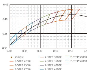
7-Step Chromaticity Quadrangles
