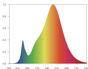
Relative Spectral Power Distribution
